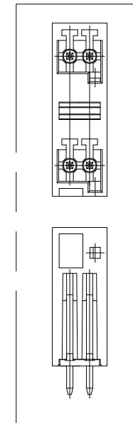
2 pole version
