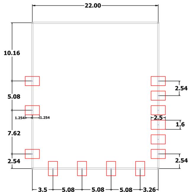
Picture 9: suggested layout for Host board
